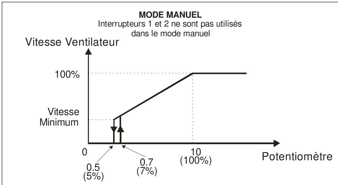
Figure 3: Diagramme logique (Mode Manuel)
