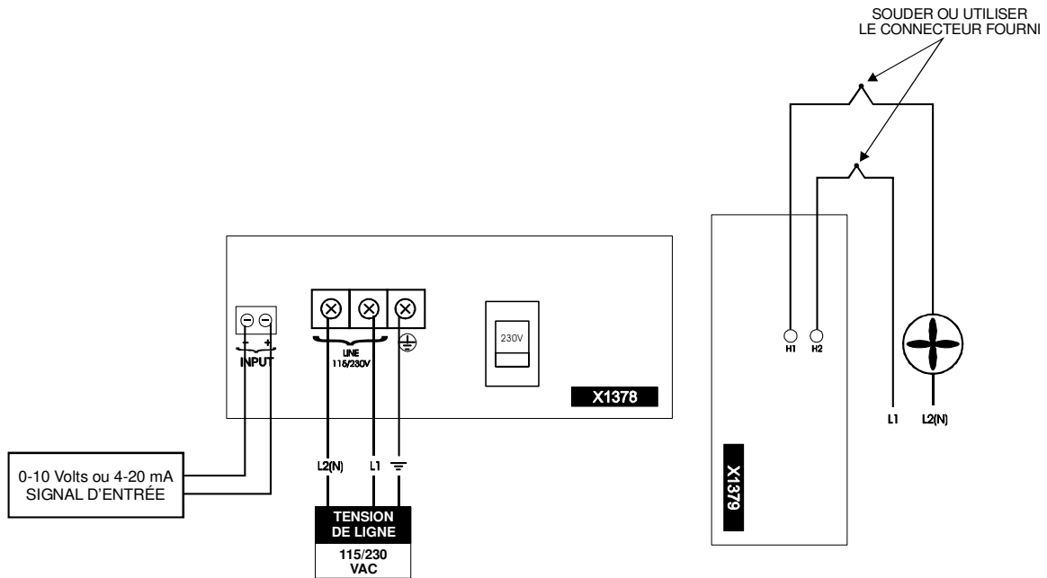
Figure 1: Diagramme de branchement
